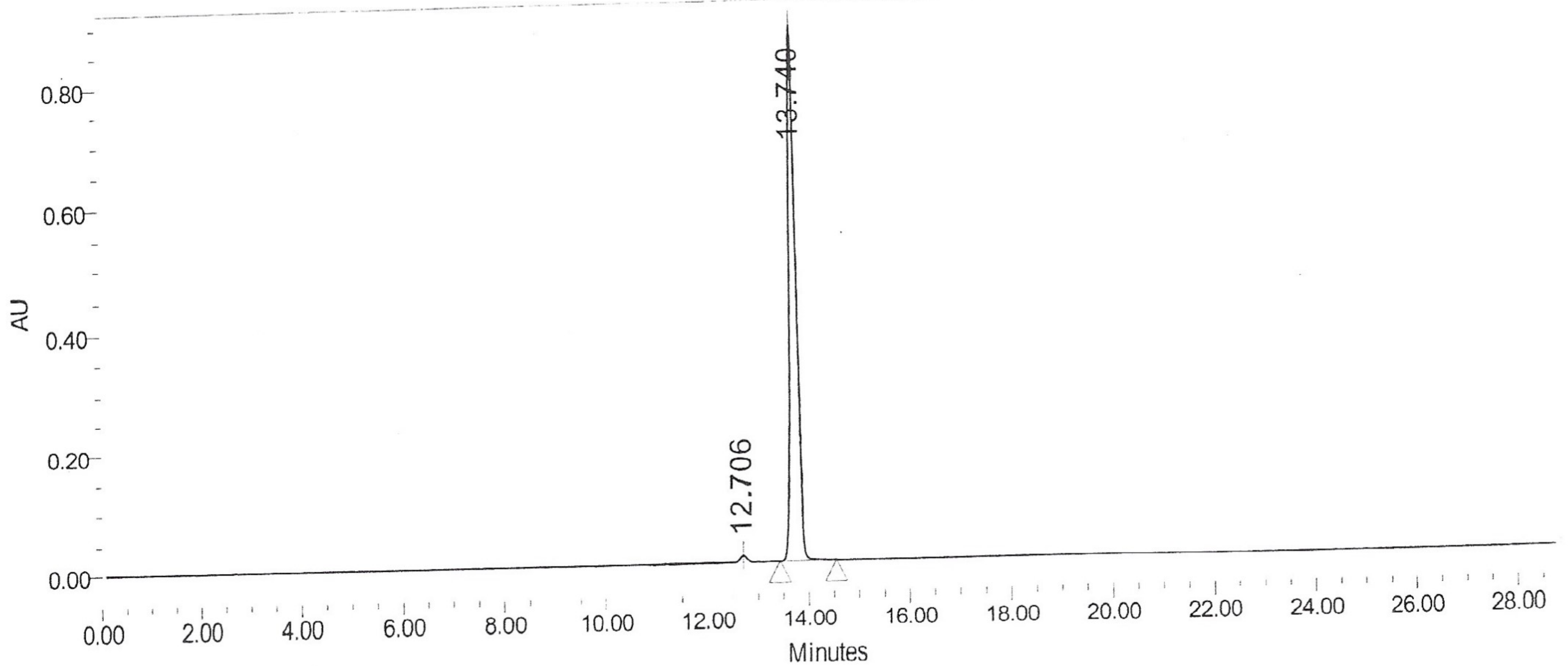
Auto-Scaled Chromatogram
